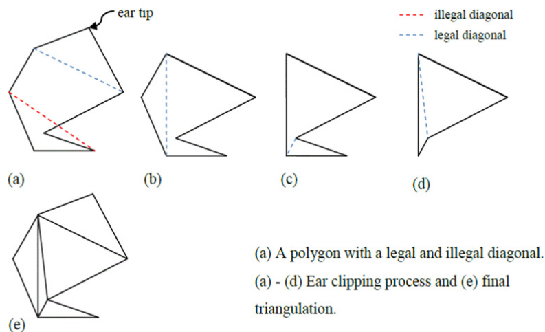
Figure 3: Ear clipping
